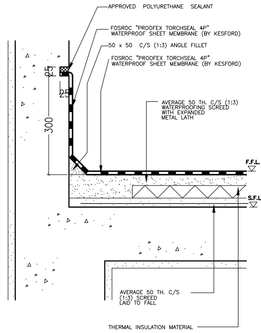
A TYPICAL ROOFING DETAIL (A2)
