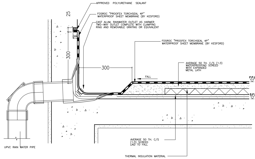
B TYPICAL DETAILS OF RAIN WATER SIDE OUTLET (A2)
