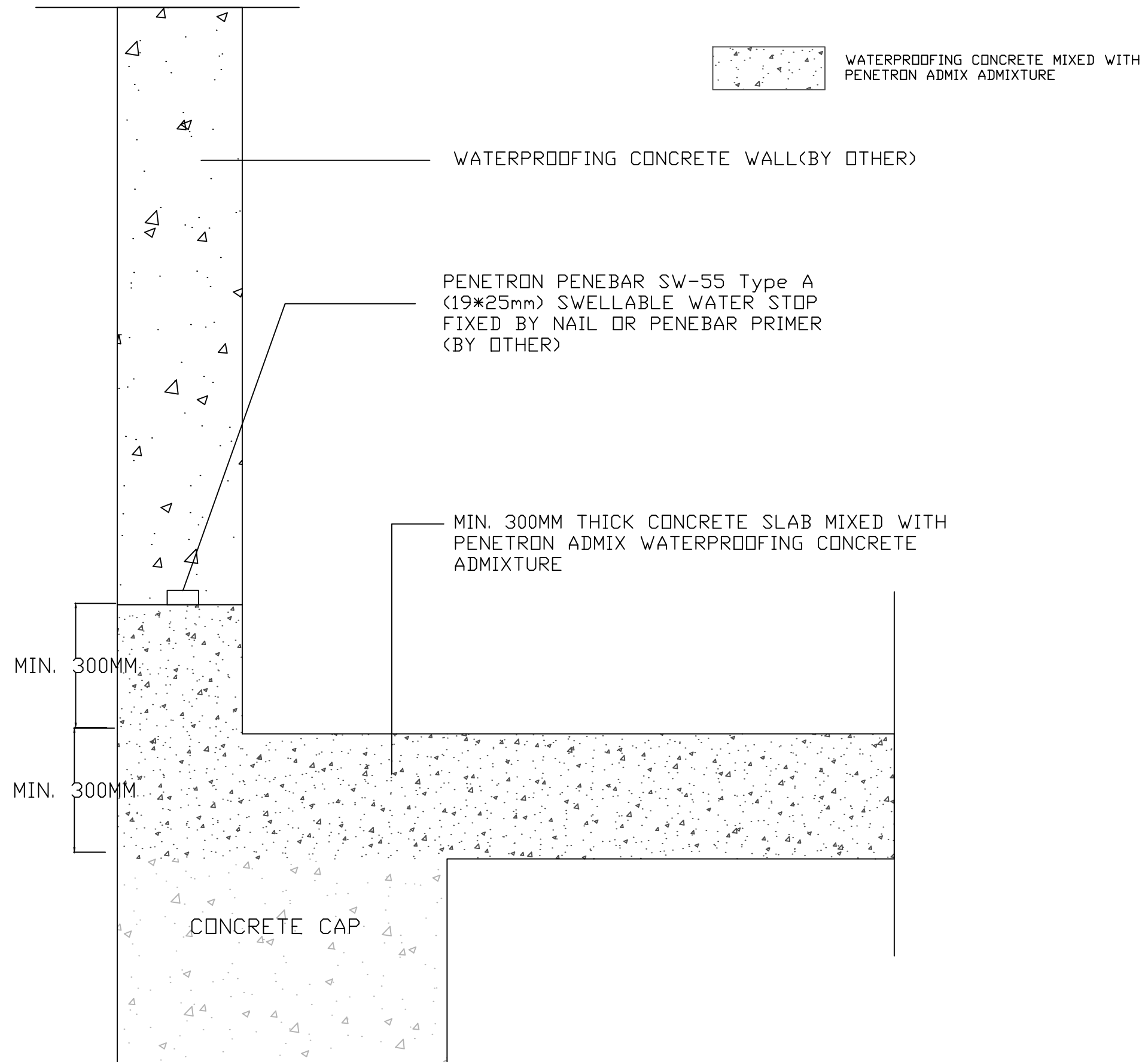
A PENETRON ADMIX WATERPROOFING DETAIL - BASEMENT CAP AND SLAB
