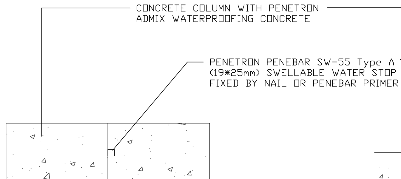
C CONSTRUCTION JOINT WATERPROOFING DETAIL FLOOR TO FLOOR
