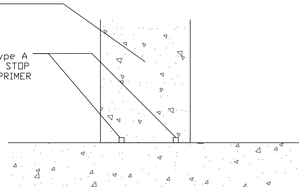
D CONSTRUCTION JOINT WATERPROOFING DETAIL CAP TO COLUMN
