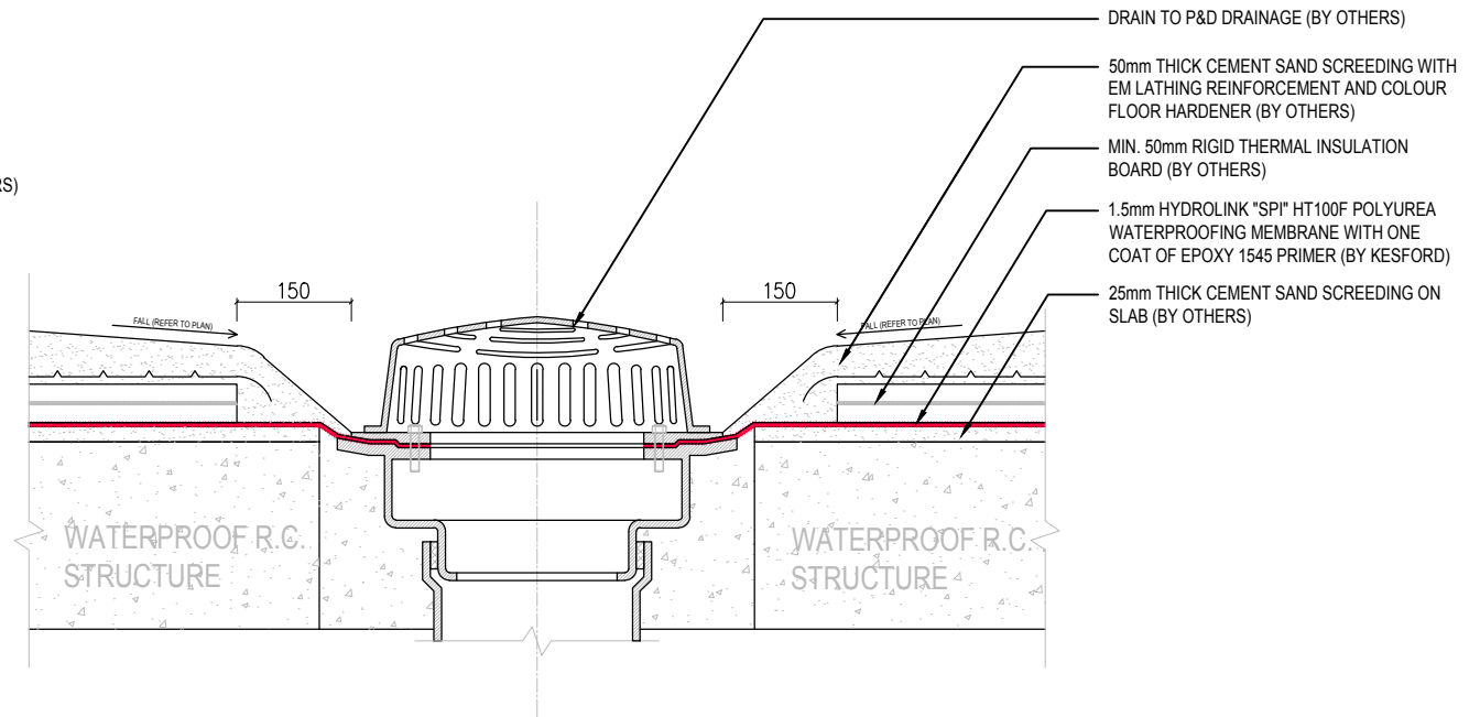
B TYPICAL ROOF DRAIN DETAIL
