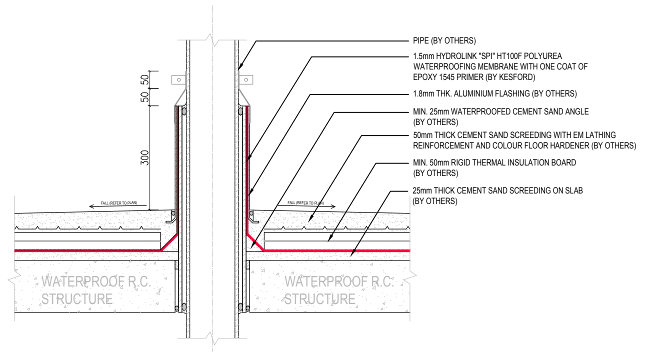
D PIPE THROUGH SLAB
