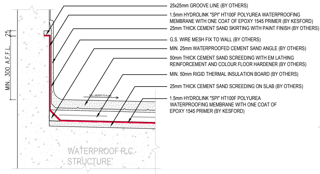
A PARAPET WALL
