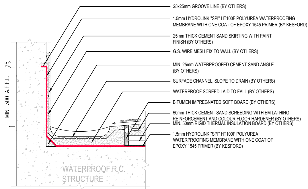
C SURFACE CHANNEL
