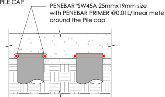
DETAIL AT PILE CAP
