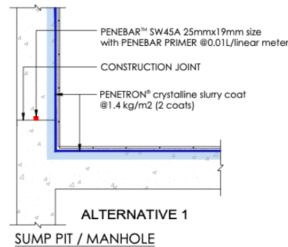
ALTERNATIVE 1 SUMP PIT / MANHOLE
