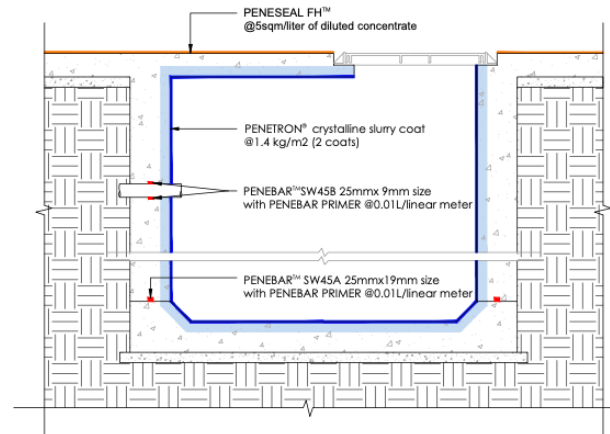
DETAIL AT PILE CAP
