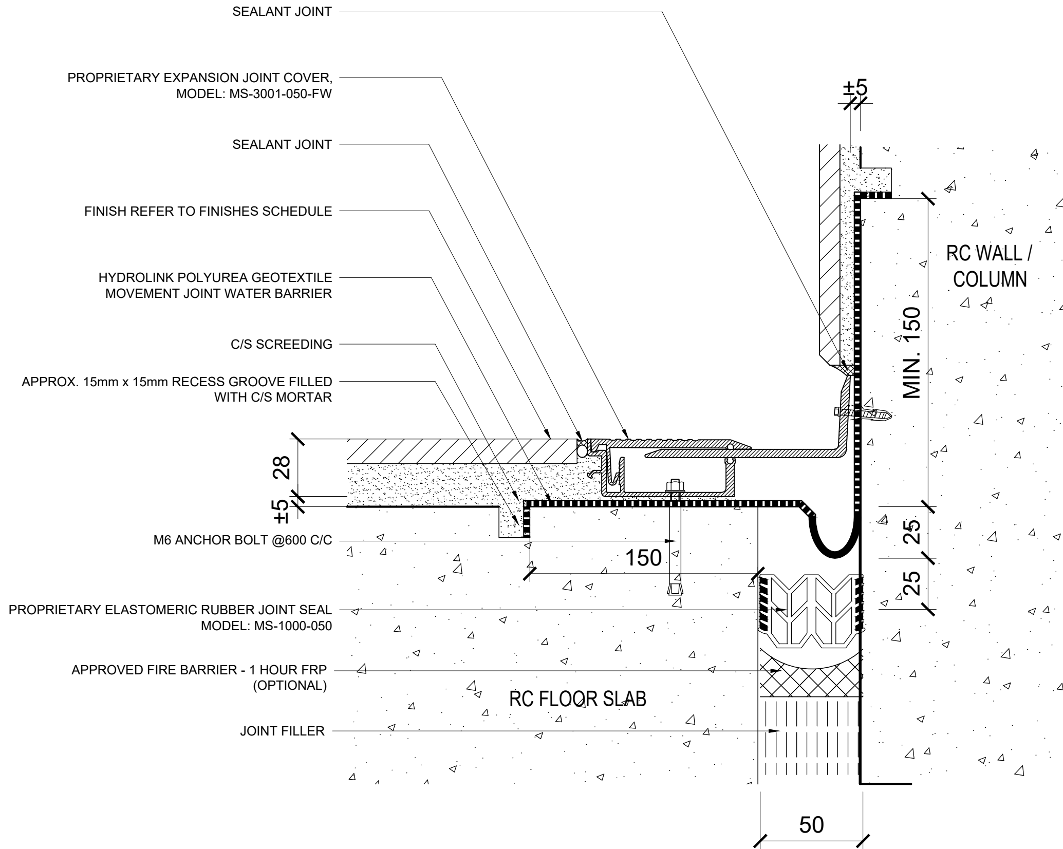
4 PROPRIETARY SEISMIC LOCK METAL MOVEMENT JOINT COVER SYSTEM MODEL NO.: HI-LINK MS-3001-50 (FLOOR TO WALL)
